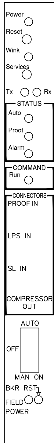
FACE PLATE
