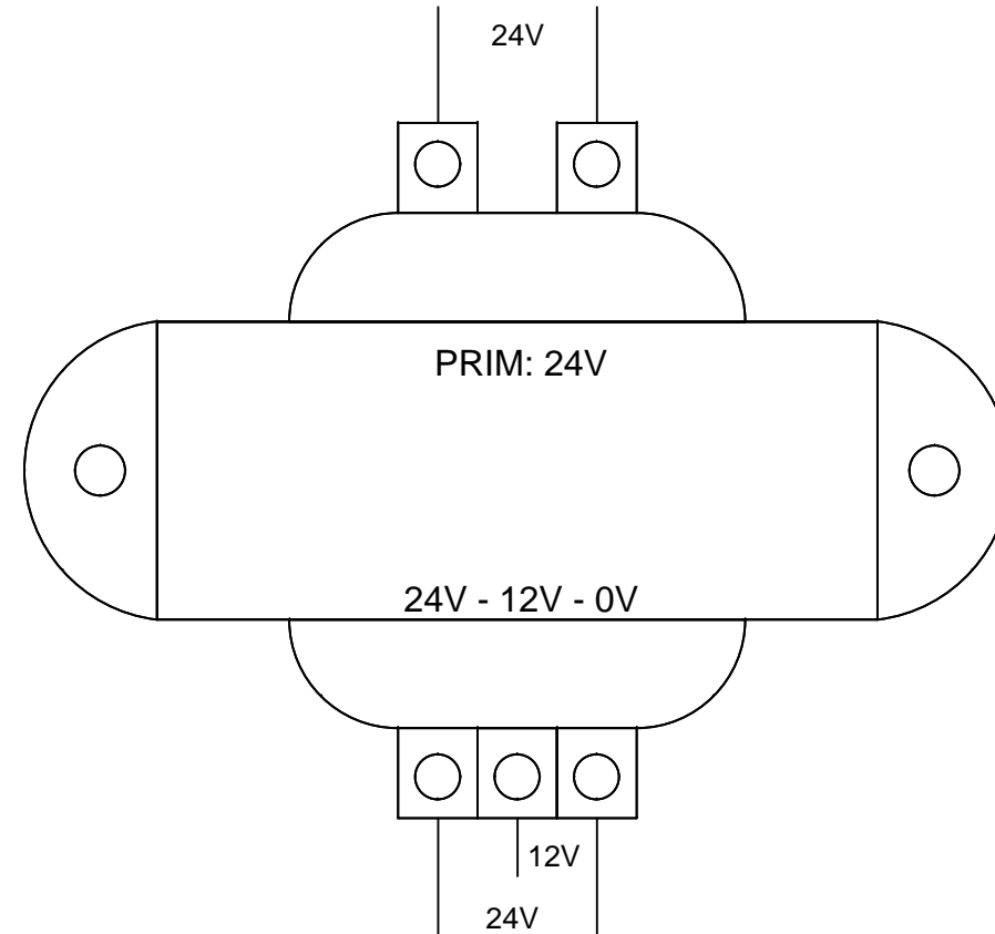
TRANSFORMER 24V to 24VCT 40VA OPEN SCREW TERMINAL
