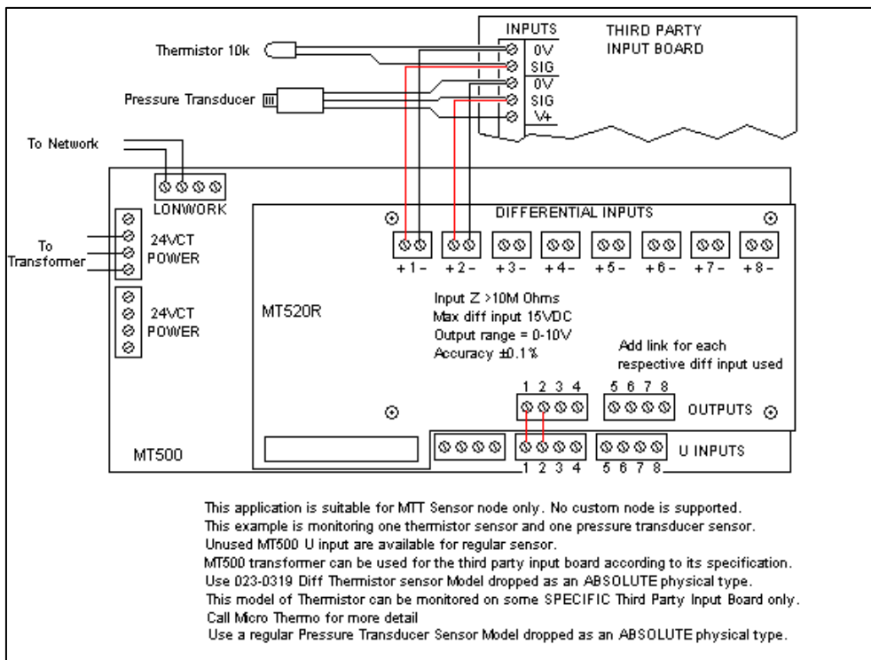
Diff Input diagram Type2.bmp
